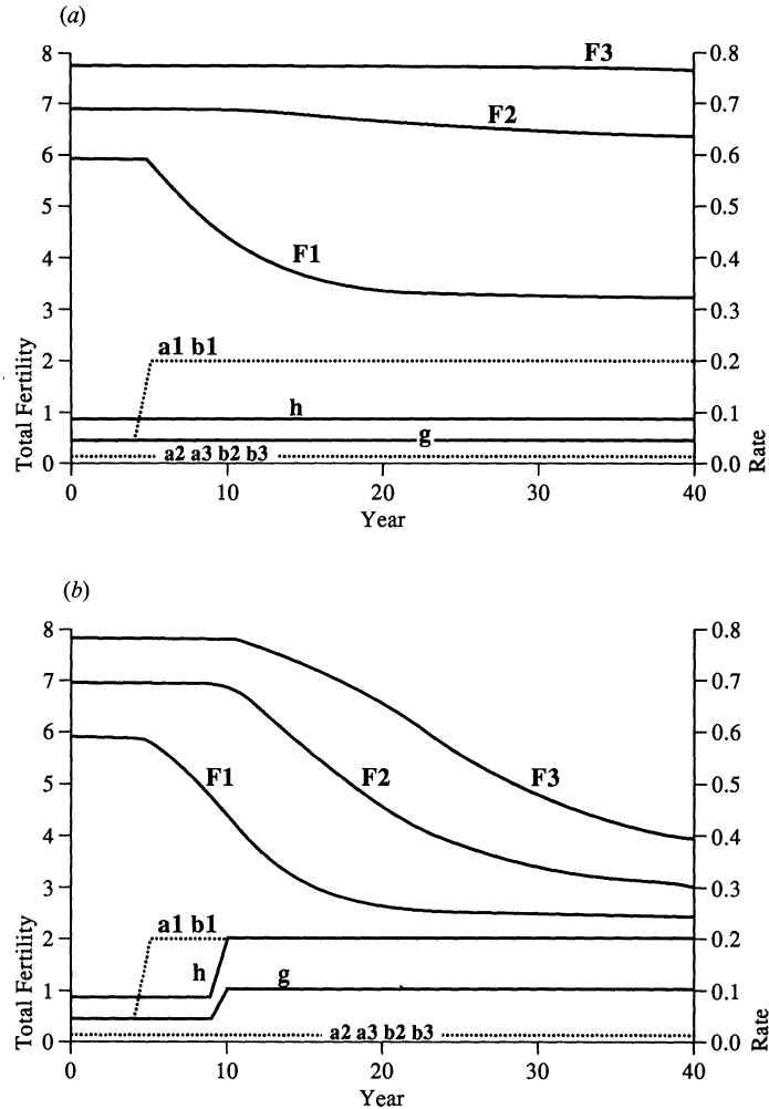
Figure 8. Simulating fertility transition trickle-down effects through three strata. Heterogeneous mix, interaction diffusion model. (a) Constant contact rates; (b) increasing contact rates.
