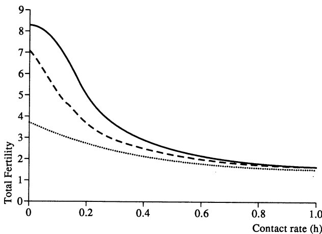
Figure 5. Effects of contact rate on fertility level at equilibrium. Simulations with the interaction diffusion model. —, a = 0.02 , b = 0.02 ; ---, a = 0.02 , b = 0.20 ; ····, a = 0.20 , b = 0.20 .
